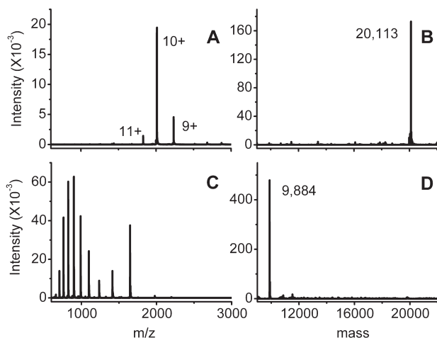
Figure 1. Electrospray ionization mass spectra, panels A and C, and deconvolutions, panels B and D: (A, B) 10 μM mitoNEET, 10 mM ammonium acetate, pH 8.5; (C, D) 10 μM mitoNEET treated with formic acid and acetonitrile for 3 h at room temperature.
