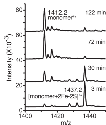
Figure 3. Electrospray ionization mass spectra, 10 μM mitoNEET, 10 mM ammonium acetate, pH 5.1, incubated for the indicated times on ice.
