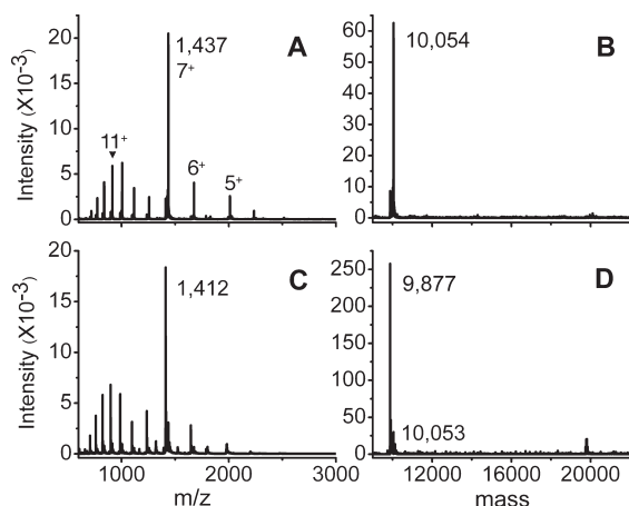
Figure 2. Electrospray ionization mass spectra, panels A and C, and deconvolutions, panels B and D: (A, B) 10 μM mitoNEET, 10 mM ammonium acetate, pH 5.1, measured immediately; (C, D) solution from (A, B) measured after 2 h on ice.
